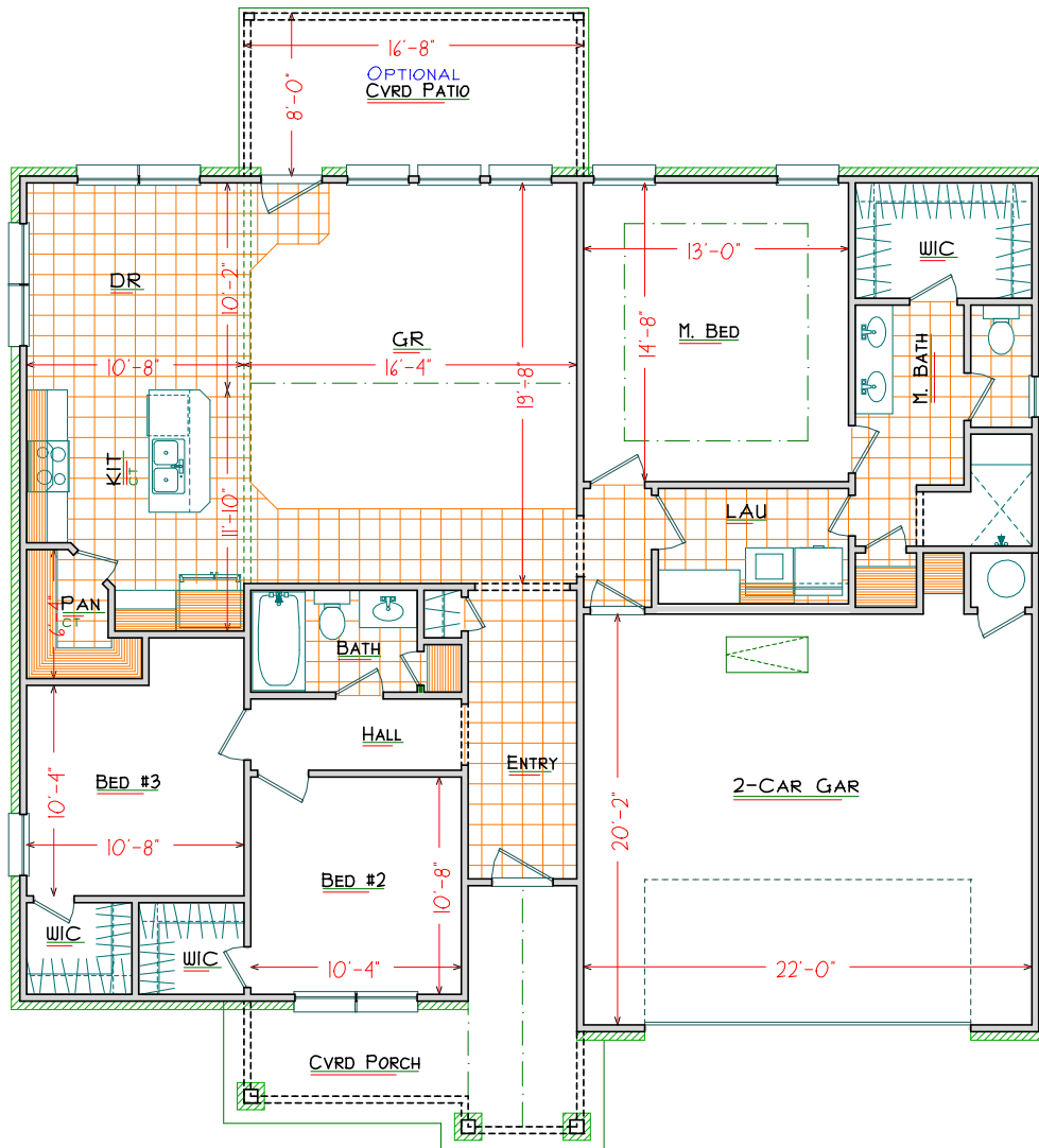
FLOOR PLAN
